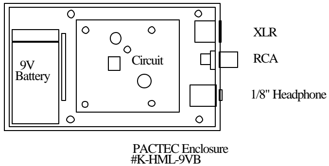
Amp/Power Unit
