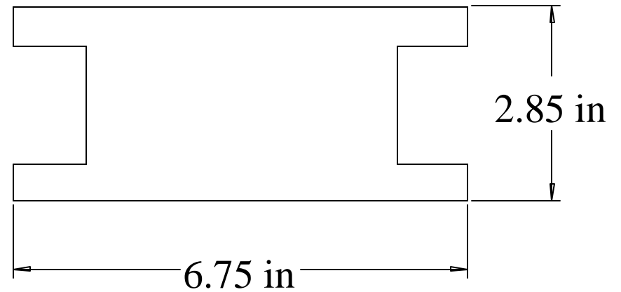
Hydrophone Reel 1/2" smooth-faced plywood
